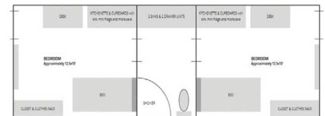
Sample room layout for Academic Standard Room type. Choose between Academic Standard, Trades Standard, Large Accessible, and Large Standard room types.
